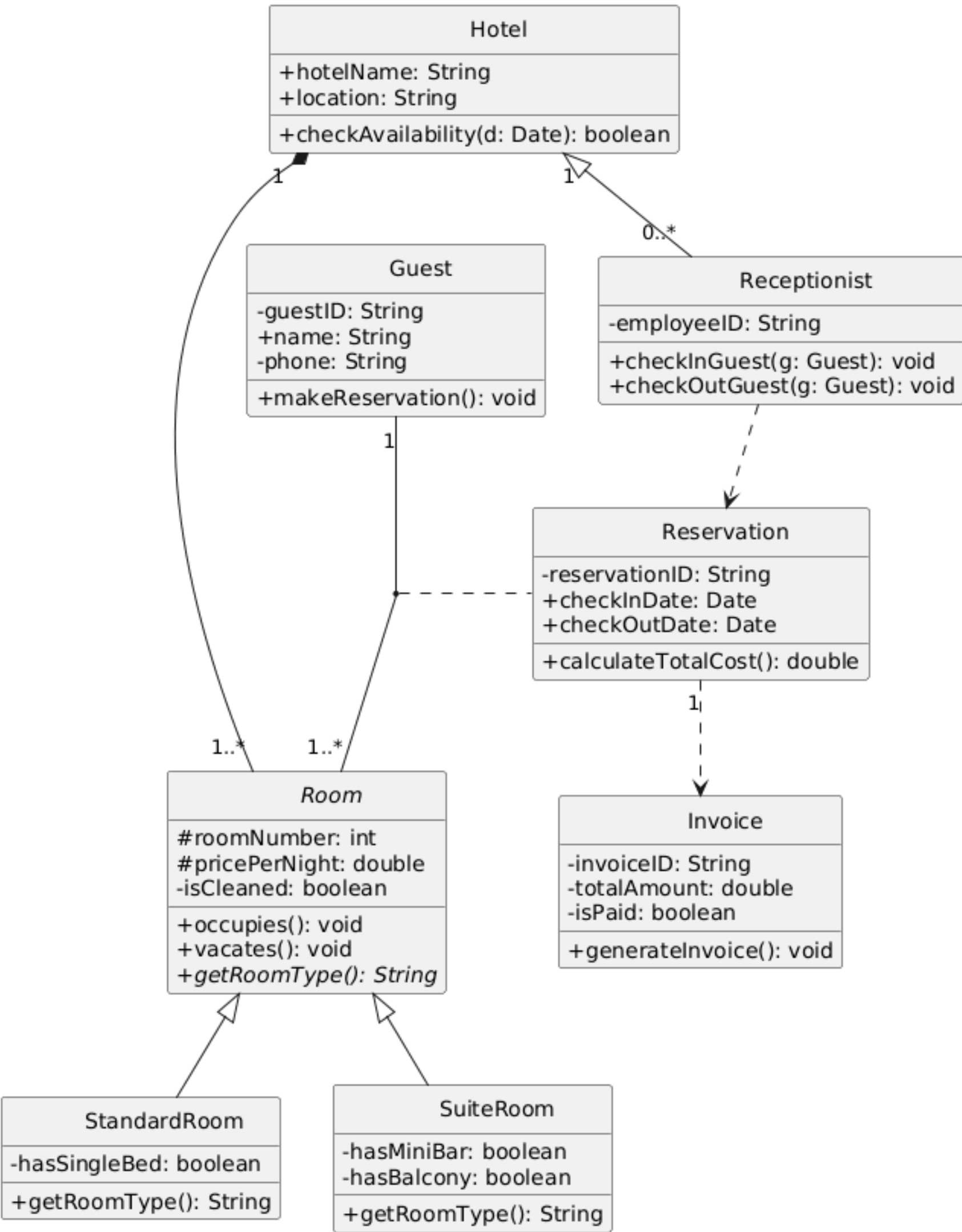
Hotel Management System - Class Diagram
